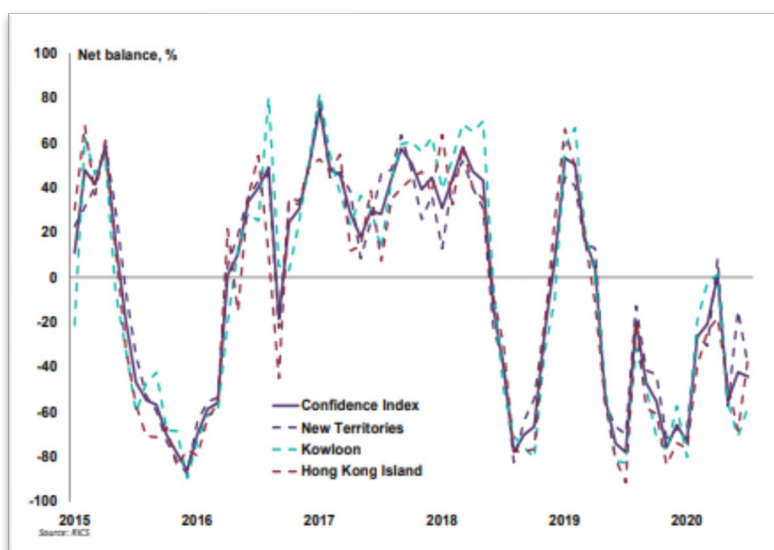
Chart 1: Confidence Index*:
