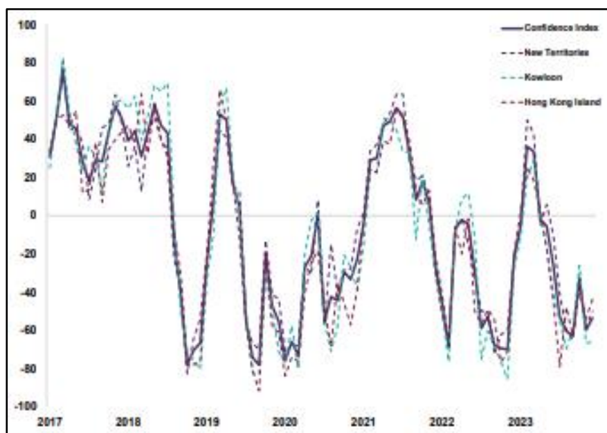
Chart 1: Confidence Index*:
